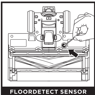
FLOORDETECT SENSOR
